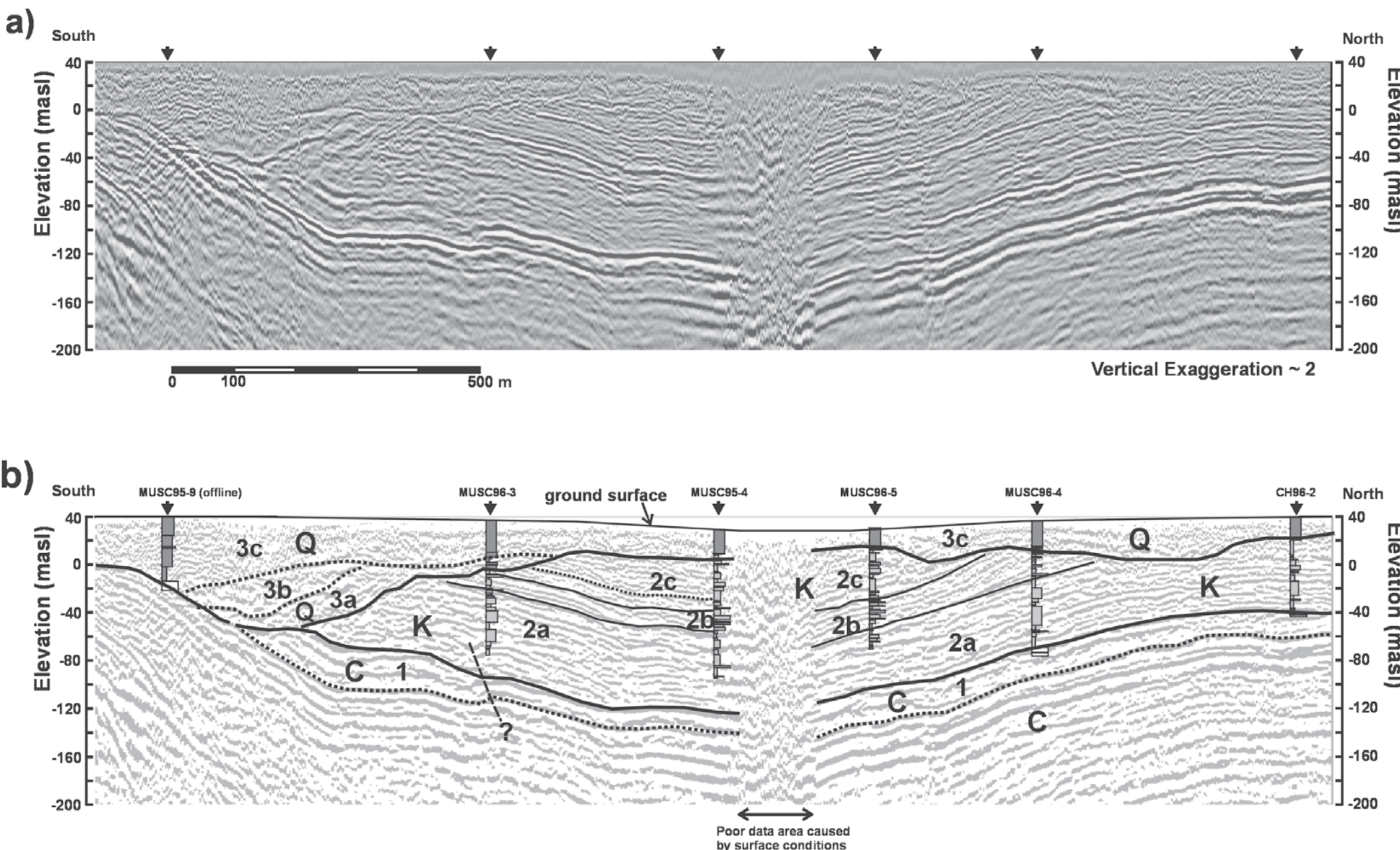
Figure 3. Type section: drill holes and reflection seismic profile of the Chaswood Formation, Elmsvale Basin after Stea and Pullan, 2001. 2a-Lower Member, 2b-Middle Member 2c-Upper Member Q-Quaternary K-Cretaceous C-Carboniferous.
